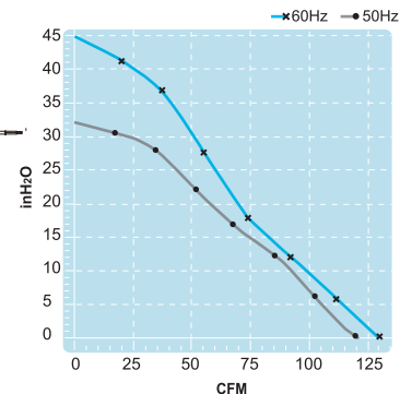
(Blower Fan)
