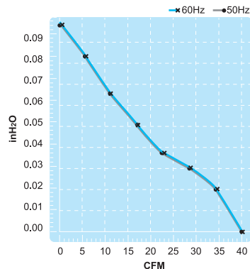
(Axial Fan)
