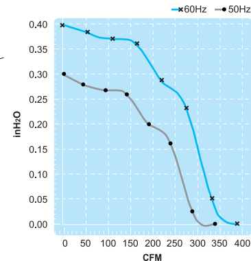
(Axial Fan)
