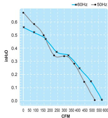
(Axial Fan)
